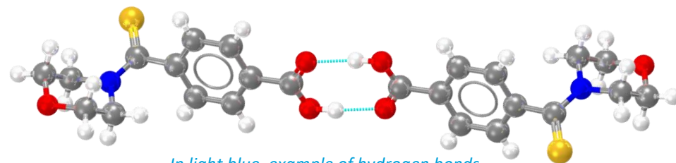
In light blue, example of hydrogen bonds for refcode MULWIC.
